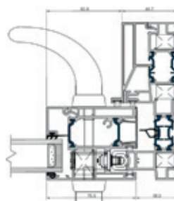
Outer Frame & Sash
