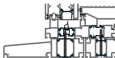
150mm Sill & Add-on
